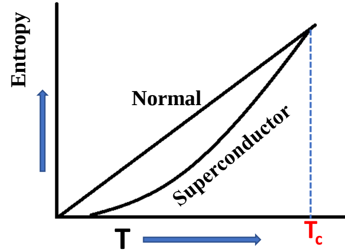
Entropy Vs Temperature(T) for Normal and superconductor
