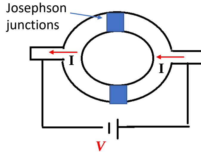
Schematic diagram of a SQUID . I is the current and V is the applied voltage
