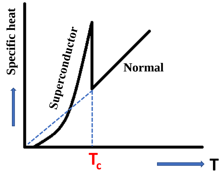
Variation of specific heat with temperature
