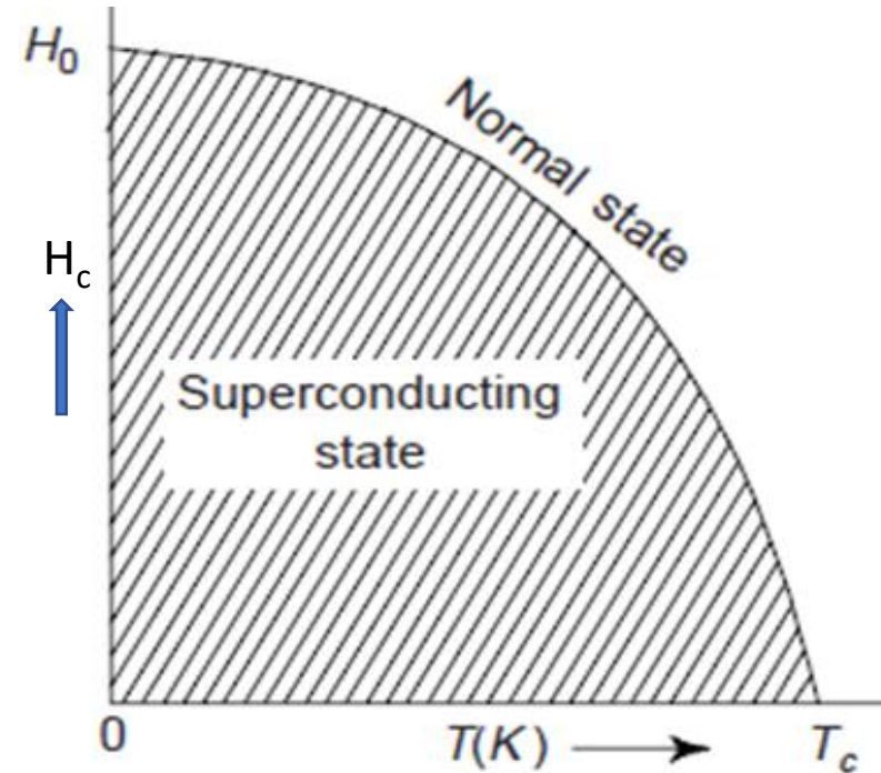
Variations of Critical Magnetic field with Temperature
